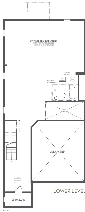
WALK-OUT CONDITION BASED ON GRADING
