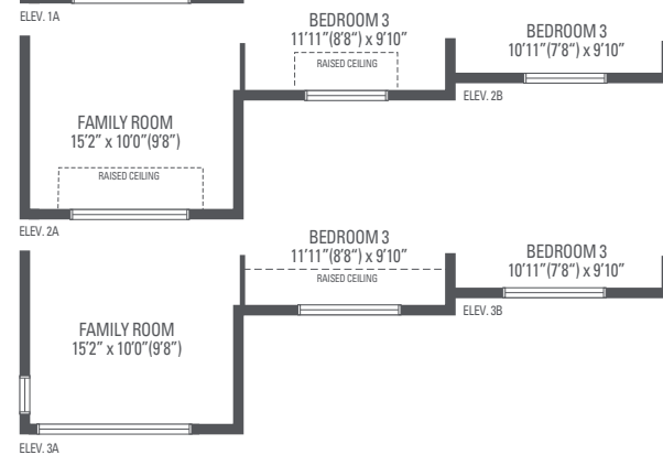
UPPER LEVEL
