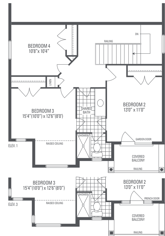
OPTIONAL 4 BEDROOM UPPER LEVEL LOFT
