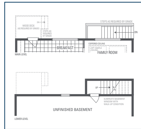
OPTIONAL UNCOVERED WALK-UP BASEMENT STAIR
