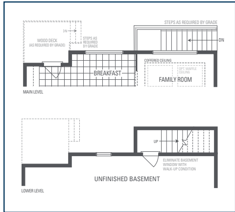
OPTIONAL UNCOVERED WALK-UP BASEMENT STAIR
